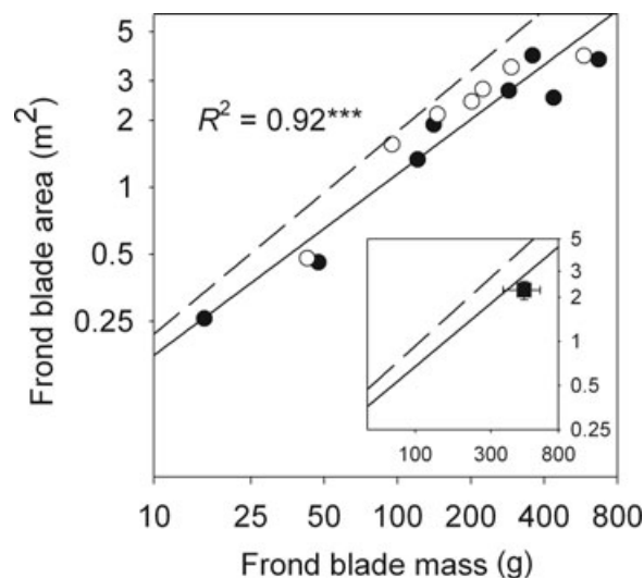
FIGURE 2. Allometries for Cibotium glaucum frond blade area versus mass, and comparison with global trends for leaf design. The solid line represents the standard major axis (SMA) for C. glaucum : \log(\text{area}) = -1.57 + 0.814 \times \log(\text{mass}) , and the dotted line represents the global intraspecific trend for leaves varying in size on mature plants of 157 angiosperm species with much smaller leaves, < 0.03 m 2 (SMA slope from Milla & Reich 2007, with intercept of C. glaucum used; see text for discussion); inset: square represents average value for C. glaucum fronds, and solid and dotted lines represent the extrapolation of global interspecific trends determined, respectively for much smaller leaves of 70 fern species up to 0.011 m 2 , and for 1943 vascular plant species up to 0.25 m 2 (for ferns, \log[\text{leaf area}] = 2.02 + 0.904 \times \log[\text{dry mass}] ; for vascular plants, \log[\text{leaf area}] = 2.01 + 0.979 \times \log[\text{dry mass}] ; Niklas et al. 2007). Symbols as in Figure 1.
